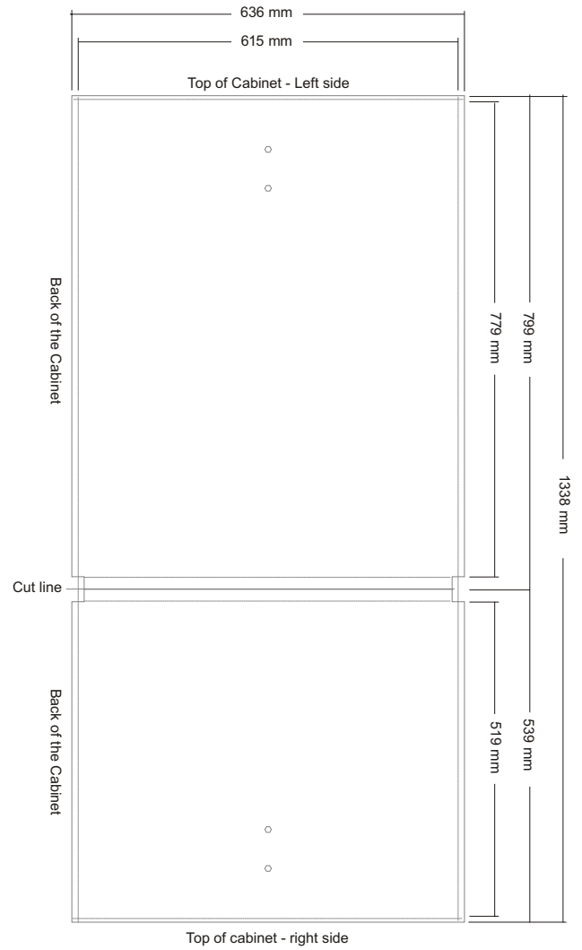
Sidewalls
